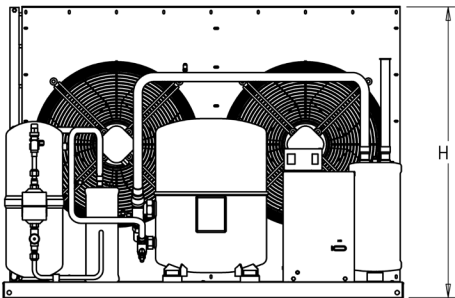
Base Type D (front and top view)
